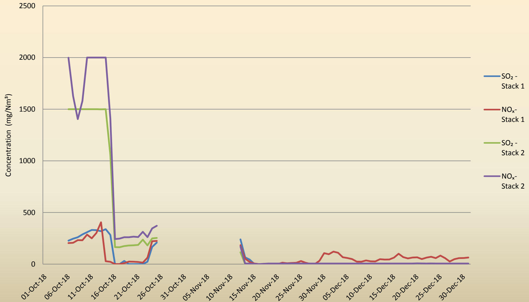
Annual Emission Trend of Gaseous in M/s. Essar Power M. P. Ltd., Dist. Singrauli (M.P.)
